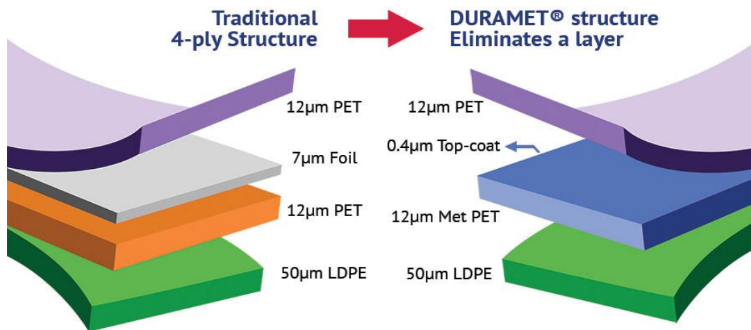
DURAMET® polyester on the right versus traditional 4-ply structure
