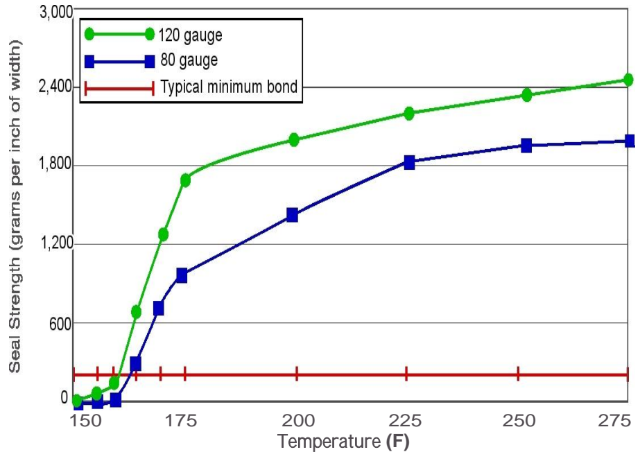
PLA Packaging Film Seal Strength vs. Temperature 20 psi and 0.25 seconds dwell time
